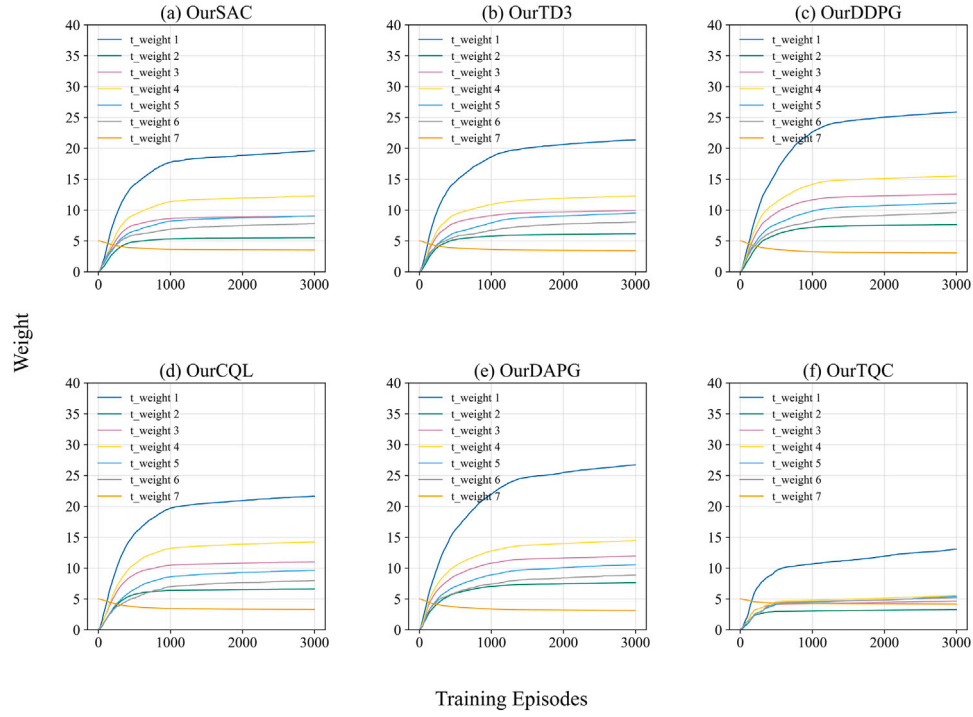
Fig. 8. Evolution curves of the reward weights for potential collision modules and the end-effector module during training under the TL-ARS-TDKDQ framework in adaptive motion planning for robotic manipulators.
