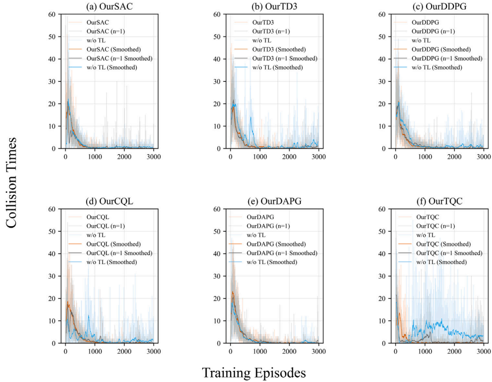
Fig. 13. Evolution of per-episode collision numbers for motion planners in dynamic robotic manipulation tasks under ablation settings of the Trend Learning module, including structural ablation (with/without TL) and temporal context ablation ( n = 1 ).
