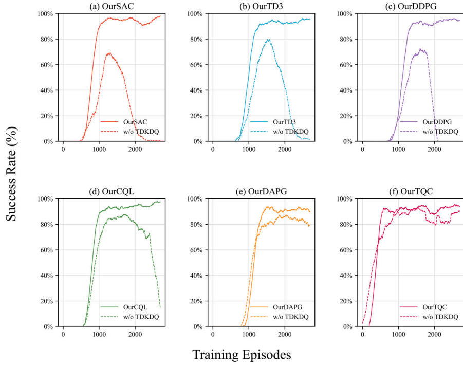
Fig. 26. Evolution of training success rates with and without the TD Error-based Q-Value Distillation module in adaptive robotic motion planning tasks under dynamic environments.
