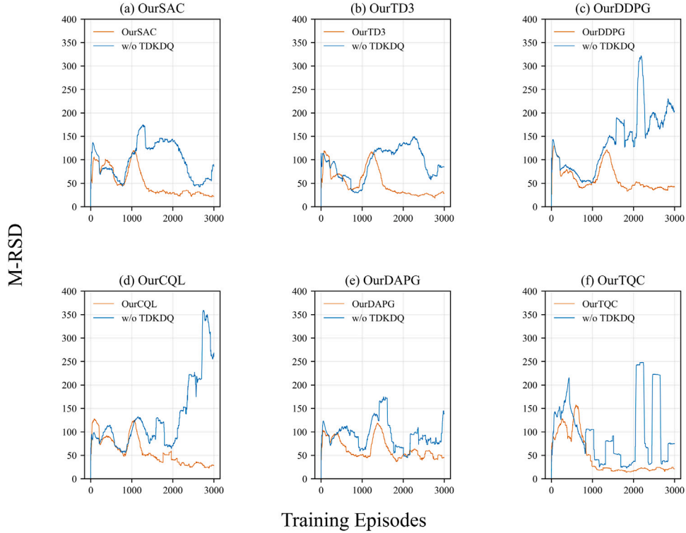
Fig. 27. Evolution of sliding-window reward standard deviations with and without the TD Error-based Q-Value Distillation module in adaptive robotic motion planning tasks under dynamic environments.
