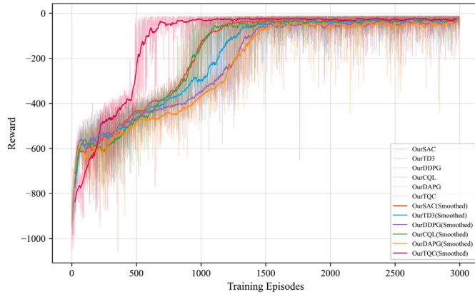
Fig. 7. Reward convergence trends of algorithms integrated with the TL-ARS-TDKDQ framework in adaptive motion planning for robotic manipulators in dynamic environments.
