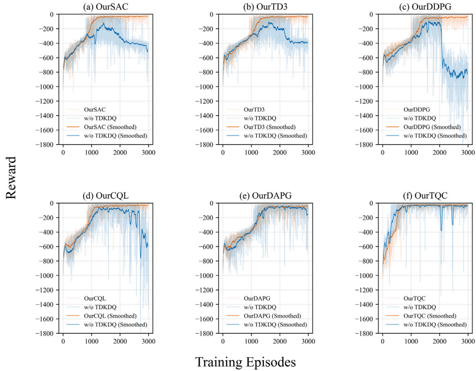
Fig. 23. Evolution of per-episode rewards with and without the TD Error-based Q-Value Distillation module in adaptive robotic motion planning tasks under dynamic environments.
