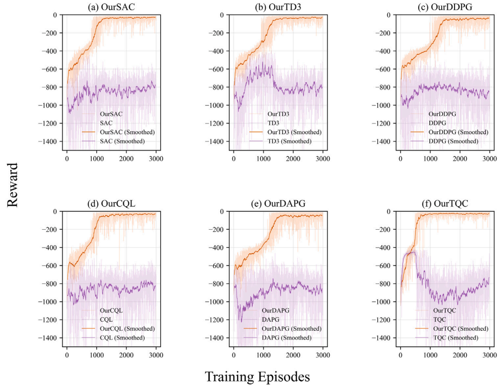
Fig. 9. Comparative analysis of reward convergence trends between algorithms integrated with the TL-ARS-TDKDQ framework and baseline algorithms in adaptive motion planning for robotic manipulators operating in dynamic environments.
