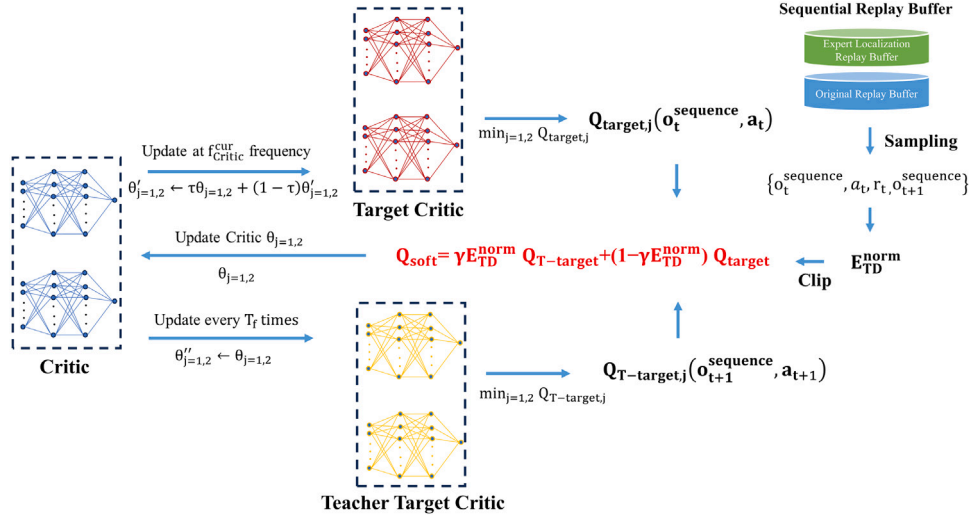
Fig. 5. This figure illustrates the update and training process for generating soft target Q-values by balancing the target Q-network and the teacher target Q-network, based on batch-normalized TD errors as evaluation indicators for non-stationary environments. During optimization, the past knowledge introduced by the teacher target Q-network effectively mitigates the risk of training collapse caused by instability in non-stationary reinforcement learning scenarios.
