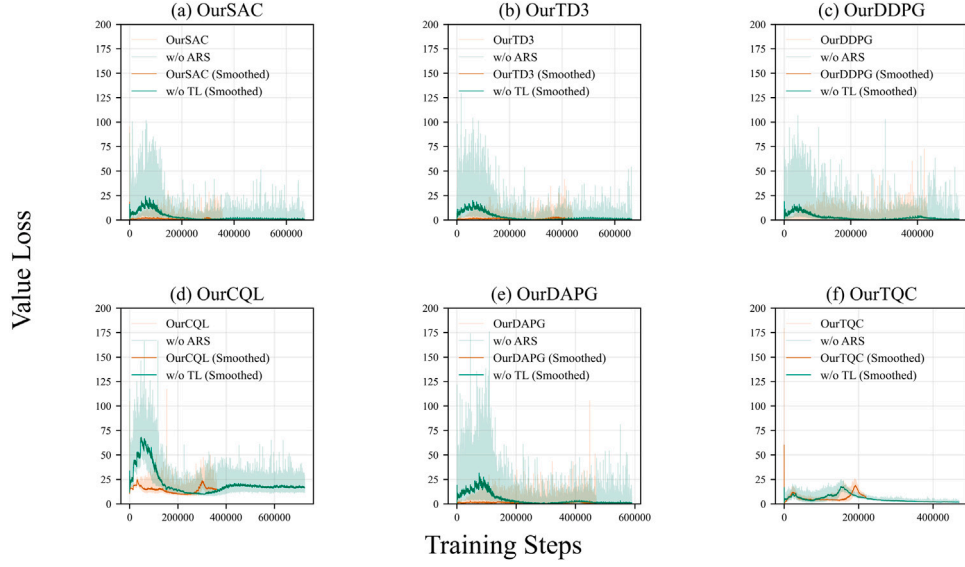
Fig. 20. Evolution of per-step value loss with and without the Adaptive Reward Shaping module in adaptive robotic motion planning tasks under dynamic environments.
