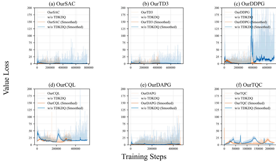
Fig. 25. Evolution of per-step value loss with and without the TD Error-based Q-Value Distillation module in adaptive robotic motion planning tasks under dynamic environments.
