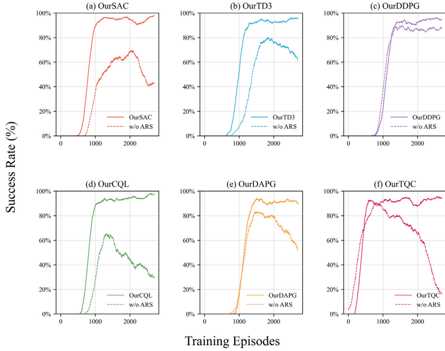
Fig. 21. Evolution of training success rates with and without the Adaptive Reward Shaping module in adaptive robotic motion planning tasks under dynamic environments.
