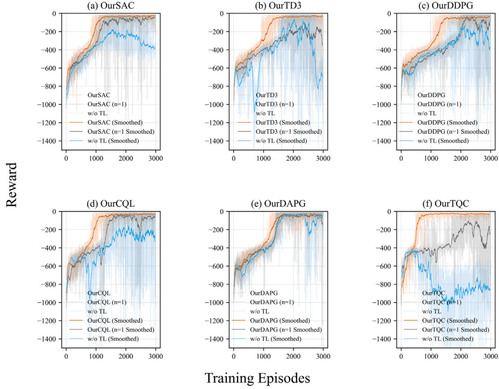
Fig. 12. Evolution of per-episode rewards for motion planners in dynamic robotic manipulation tasks under ablation settings of the Trend Learning module, including structural ablation (with/without TL) and temporal context ablation ( n = 1 ).
