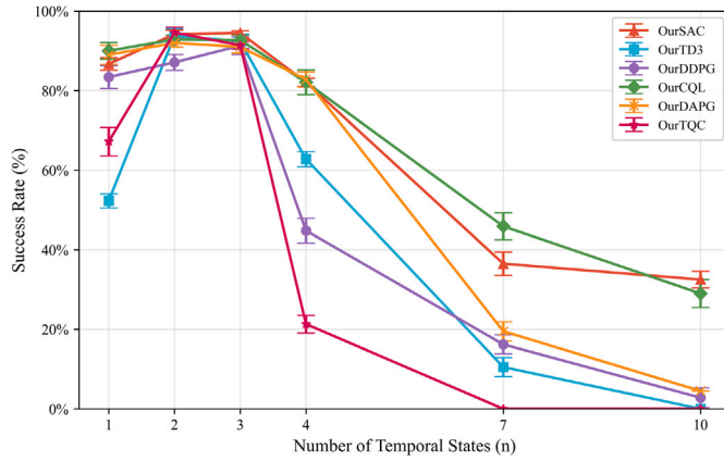
Fig. 17. Evolution of training success rates under the Trend Learning mechanism with varying temporal sequence lengths in adaptive robotic motion planning tasks.
