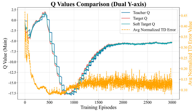
Fig. 28. Visualization of the adaptive Q-value fusion among the teacher target Q, target Q, and soft Q guided by batch-normalized TD errors.
