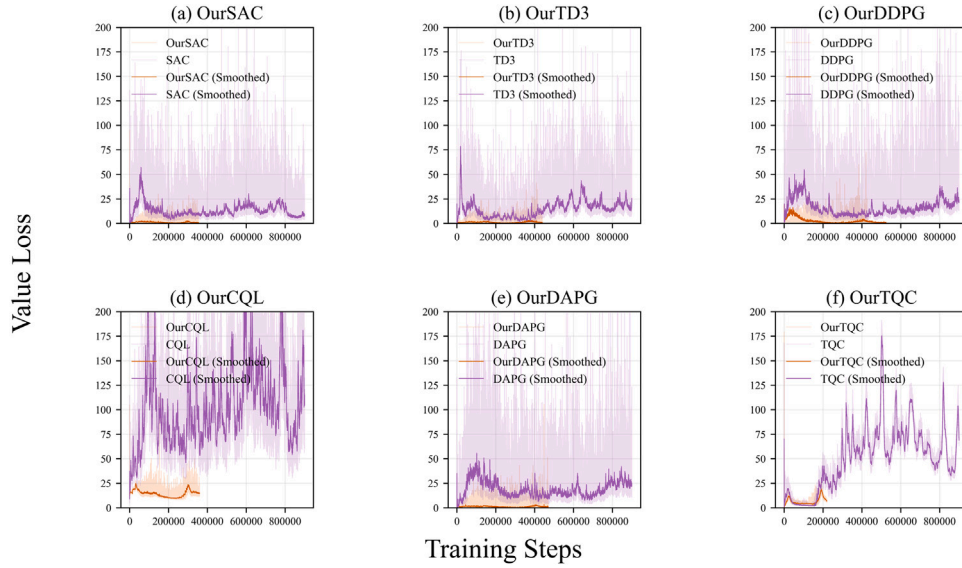
Fig. 11. Comparative analysis of value loss trends between algorithms integrated with the TL-ARS-TDKDQ framework and baseline algorithms in adaptive motion planning for robotic manipulators operating in dynamic environments.
