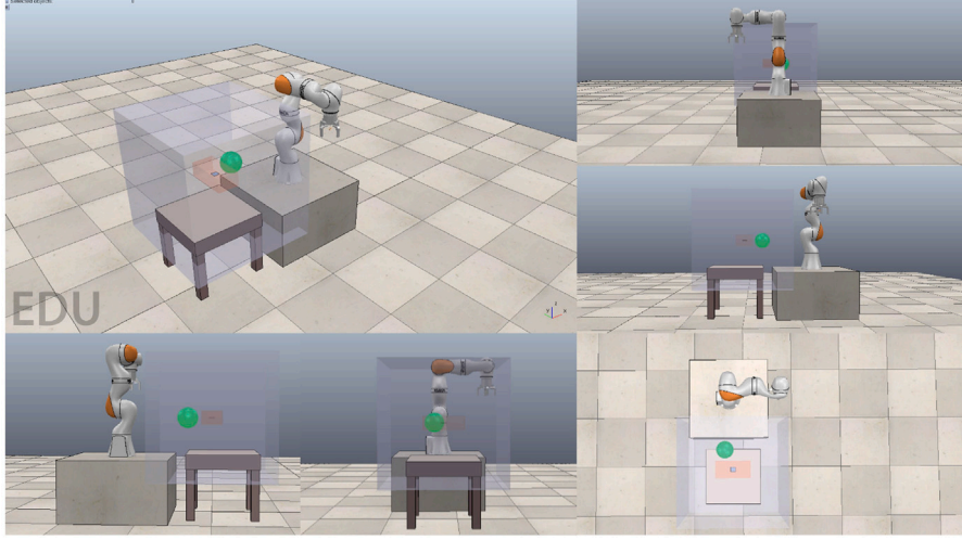
Fig. 6. Adaptive motion planning simulation environment for a robotic manipulator in a dynamic environment based on CoppeliaSim.
