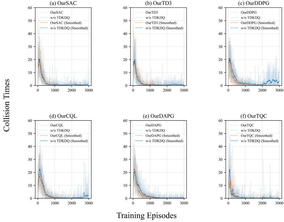
Fig. 24. Evolution of per-episode collision numbers with and without the TD Error-based Q-Value Distillation module in adaptive robotic motion planning tasks under dynamic environments.
