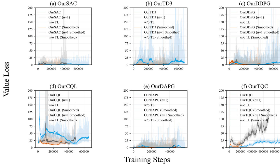
Fig. 14. Evolution of per-step value loss for motion planners in dynamic robotic manipulation tasks under ablation settings of the Trend Learning module, including structural ablation (with/without TL) and temporal context ablation ( n = 1 ).
