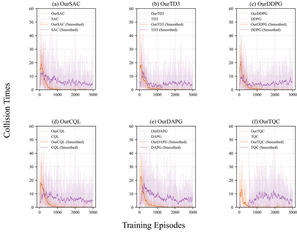
Fig. 10. Evolution curves of per-episode collision counts for potential-collision modules of robotic manipulators during adaptive motion planning, comparing the TL-ARS-TDKDQ framework with other baseline algorithms.
