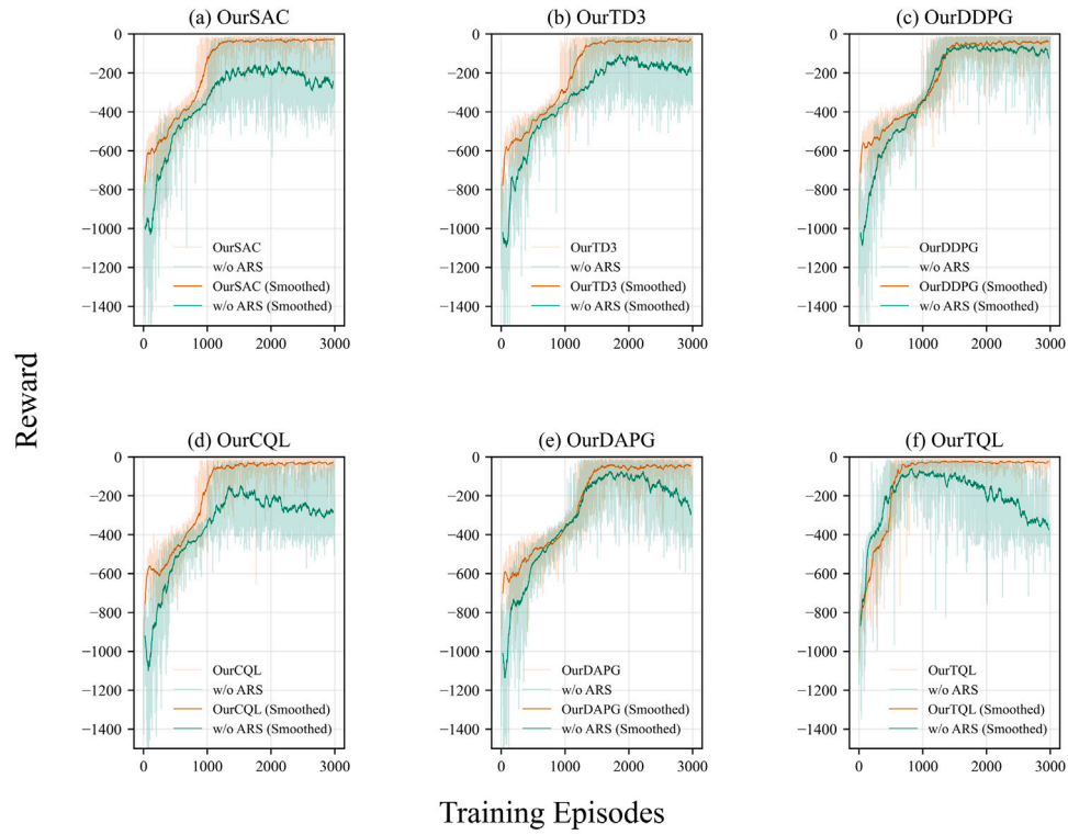
Fig. 18. Evolution of per-episode rewards with and without the Adaptive Reward Shaping module in adaptive robotic motion planning tasks under dynamic environments.
