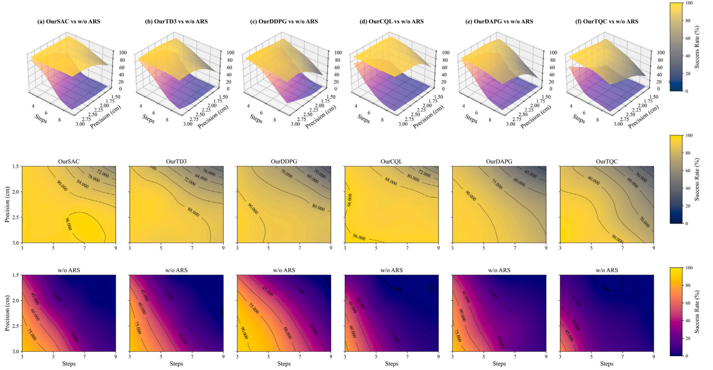
Fig. 22. Success rate comparison with and without the Adaptive Reward Shaping (ARS) module in task generalization tests for adaptive robotic arm motion planning under dynamic environments. Subfigures show 3D success-rate surfaces and the corresponding 2D heatmaps for both variants across different precision levels and step settings.
