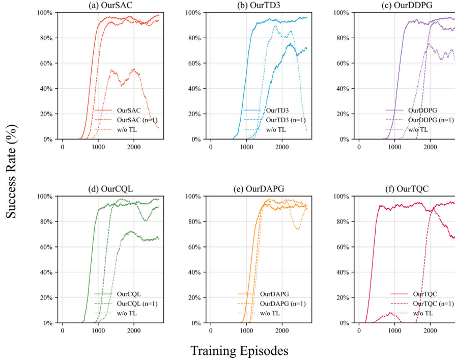
Fig. 15. Evolution of sliding-window success rates for motion planners in dynamic robotic manipulation tasks under ablation settings of the Trend Learning module, including structural ablation (with/without TL) and temporal context ablation ( n = 1 ).
