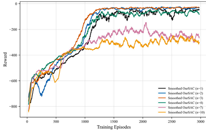
Fig. 16. Evolution of per-episode rewards under the Trend Learning mechanism with different temporal sequence lengths in adaptive robotic motion planning tasks.
