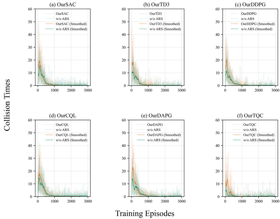
Fig. 19. Evolution of per-episode collision numbers with and without the Adaptive Reward Shaping module in adaptive robotic motion planning tasks under dynamic environments.
